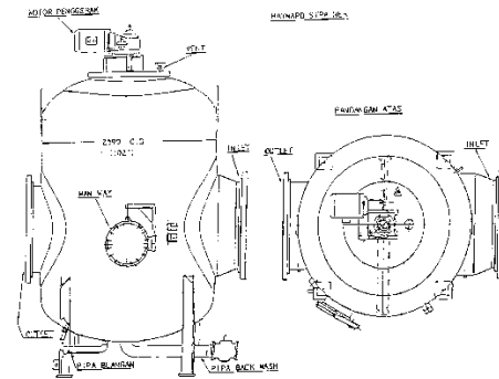
Figure 3. Hayward Strainer
