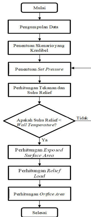
Gambar 1. Diagram alir
