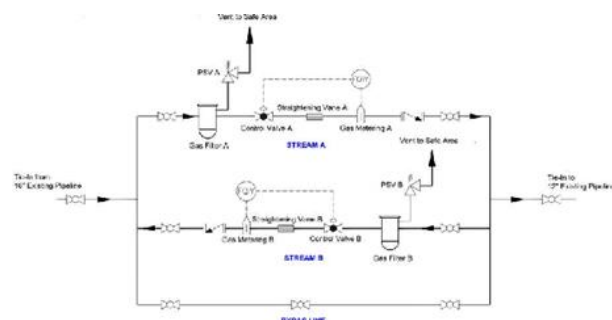
Gambar 1. Process Flow Diagram stasiun metering gas
