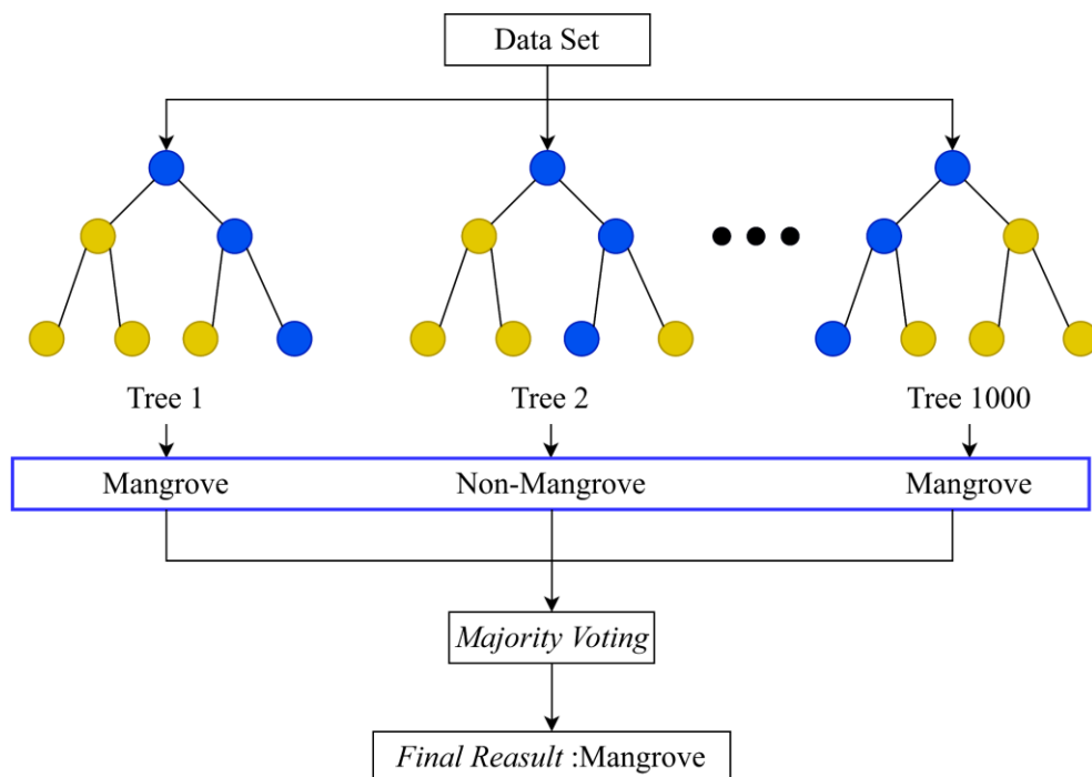
Gambar 3. Algoritma random forest
