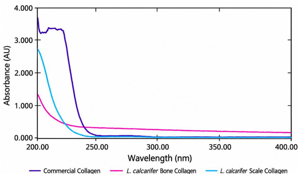
Figure 2. UV absorption spectra of bone collagen, scale collagen, and commercial collagen
