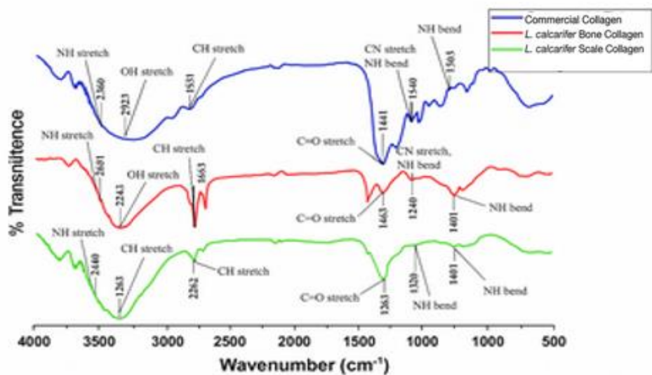
Figure 3. FTIR spectra of bone collagen, scale collagen, and commercial collagen
