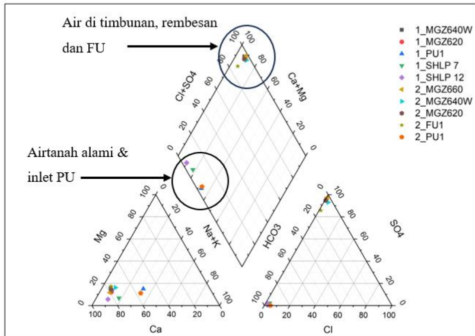
Gambar 3. Diagram Piper
