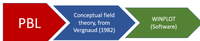
Figure 1. Methodology for research on ODEs
