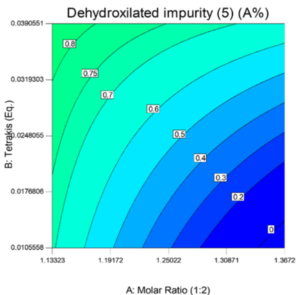
Figure 9. Effect of tetrakis and molar ratio on the dehydroxilated impurity in the contour plot.
