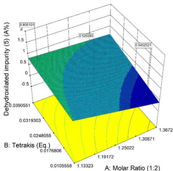
Figure 10. Effect of tetrakis and molar ratio on the dehydroxilated impurity in the surface plot.
