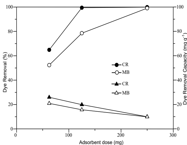
Figure 7. Effect of \text{TiO}_2/\text{SCEC} adsorbent dose on sorption of MB and CR. Conditions: (pH: 6.9, concentration MB and CR from 100 \text{mg.L}^{-1} , time 30 min, weight adsorbent: 62.5 , 125 and 250 mg, at 25^\circ\text{C} ).
