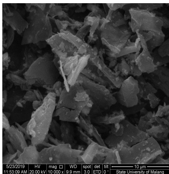
Figure 5. SEM/EDX Image of TiO 2 /SCEC adsorbent.
