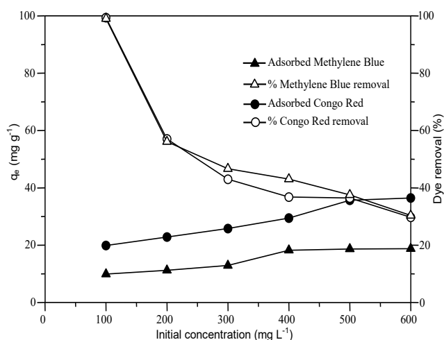
Figure 9. Effect of initial dye concentration on sorption of MB and CR on \text{TiO}_2/\text{SCEC} . Conditions: (pH: 6.9, concentration MB and CR from 100 – 600 \text{mg.L}^{-1} , weight adsorbent for MB 250 mg and CR 125 mg, at 25^\circ\text{C} ).
