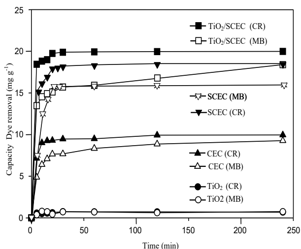
Figure 6. Effect of contact time on the amount of MB and CR dyes removal on TiO 2 ; CEC, SCEC and TiO 2 /SCEC. Conditions: (pH: 6.9, concentration MB and CR 100 mg.L -1 , weight adsorbent for MB 250 mg and CR 125 mg, at 25°C).
