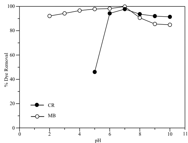
Figure 8. Effect of pH on % MB and CR dye removal on \text{TiO}_2/\text{SCEC} , Conditions: (pH: 6.9, concentration MB and CR from 100 \text{mg.L}^{-1} , weight adsorbent for MB 250 mg and CR 125 mg, at 25^\circ\text{C} ).
