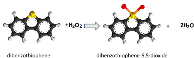
Figure 1. Oxidation desulfurization process of DBT [10]
