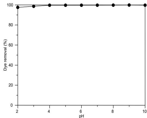
Figure 11. Effect of pH on methylene blue dye removal. Conditions: (MB: 100 \text{mg.L}^{-1} , weight adsorbent: 250 mg, at 30°C).
